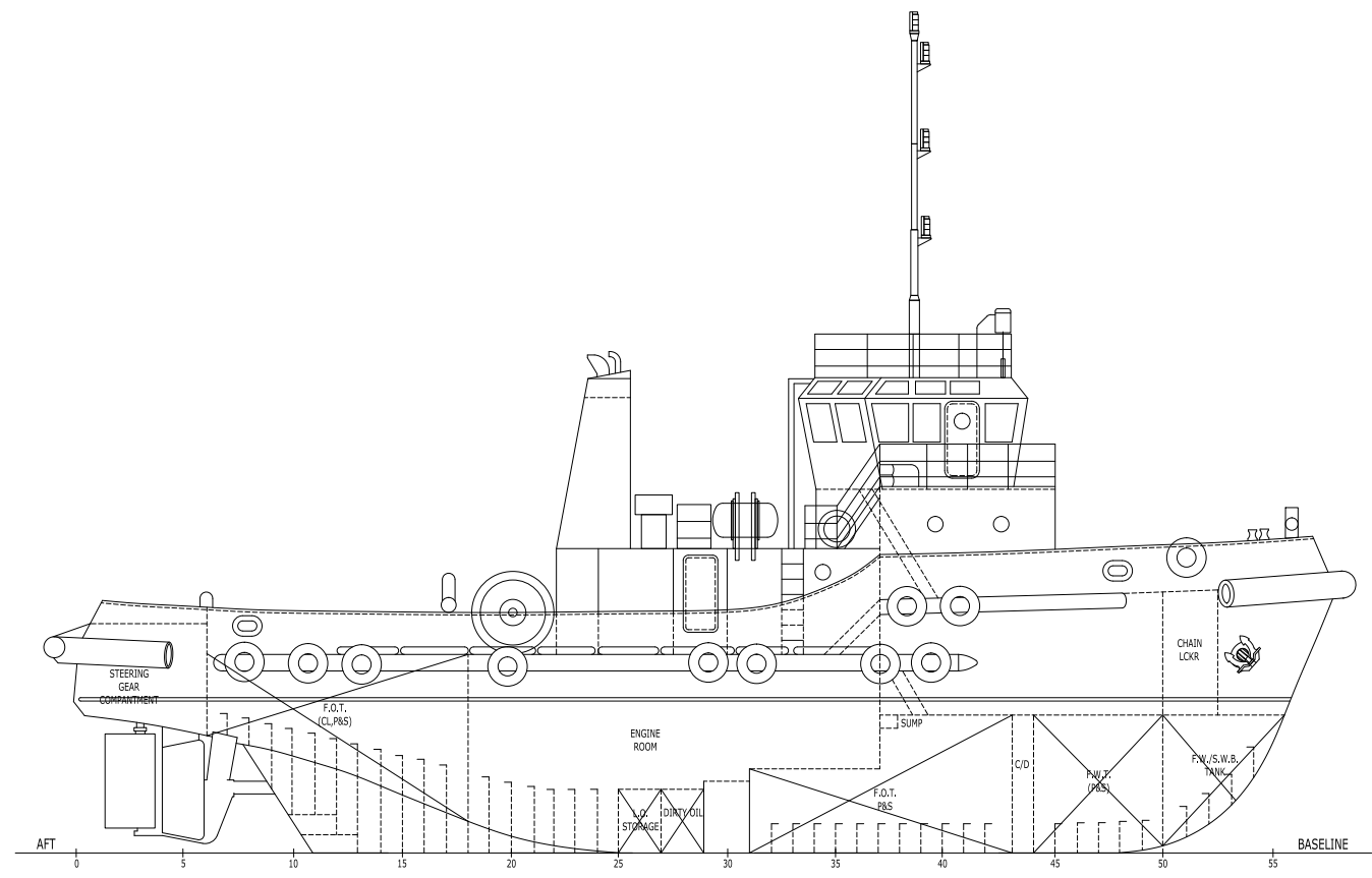
OUTBOARD PROFILE
