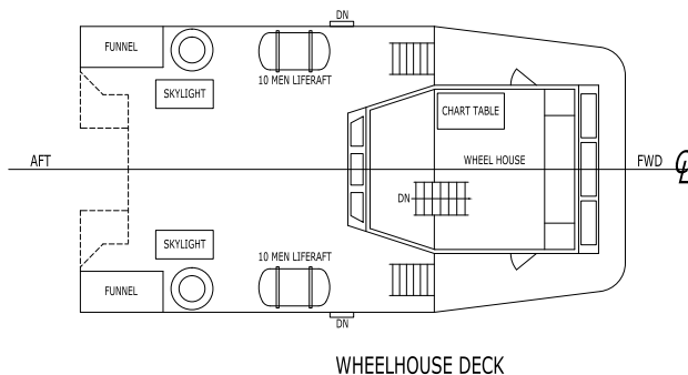
WHEELHOUSE DECK
