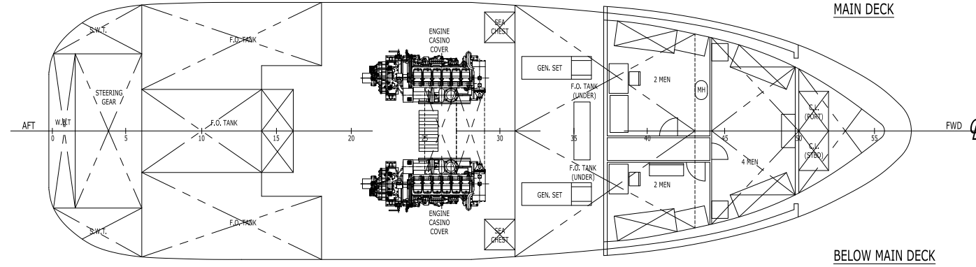
MAIN DECK
