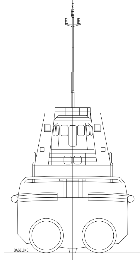
STERN VIEW
